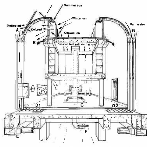
Fig 7.4 Section through a gallery
