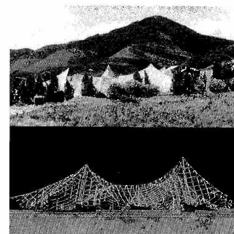
Fig 4.4 Model of hanging roof of Ice Rink, Vail, Colorado
