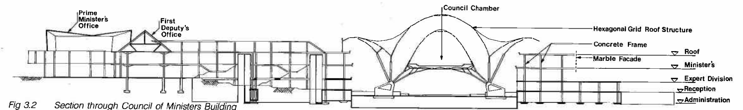
Fig 3.2 Section through Council of Ministers Building
