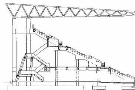
Fig 8.3 Section through stadium
