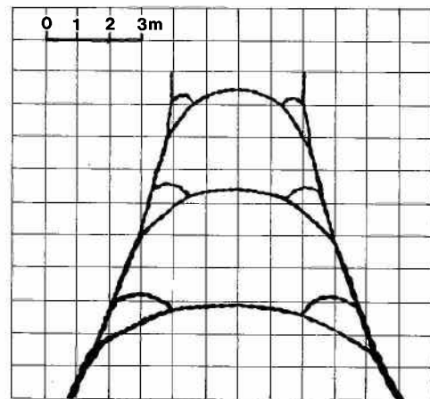
Fig 12.8 Hanging chain model for 'wall' structure
